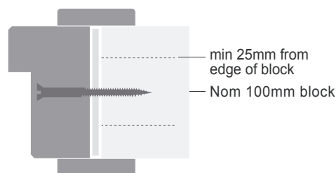
Secure fixing zone
